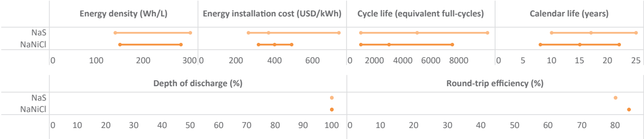
Figure 45: Properties of high temperature battery electricity storage systems, 2016
