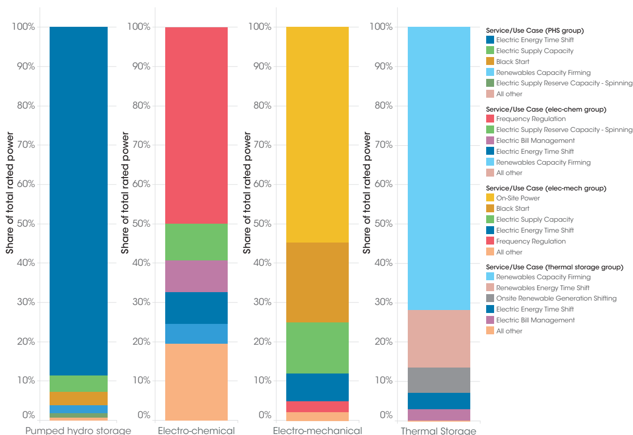
Figure 7: Global energy storage power capacity shares by main-use case and technology group, mid-2017
