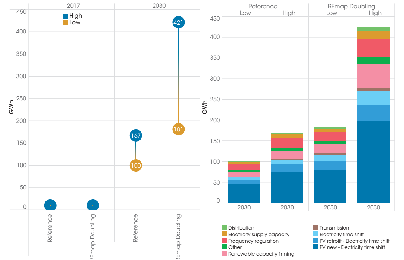
Figure 55: Battery electricity storage energy capacity growth in stationary applications by main-use case, 2017-2030
