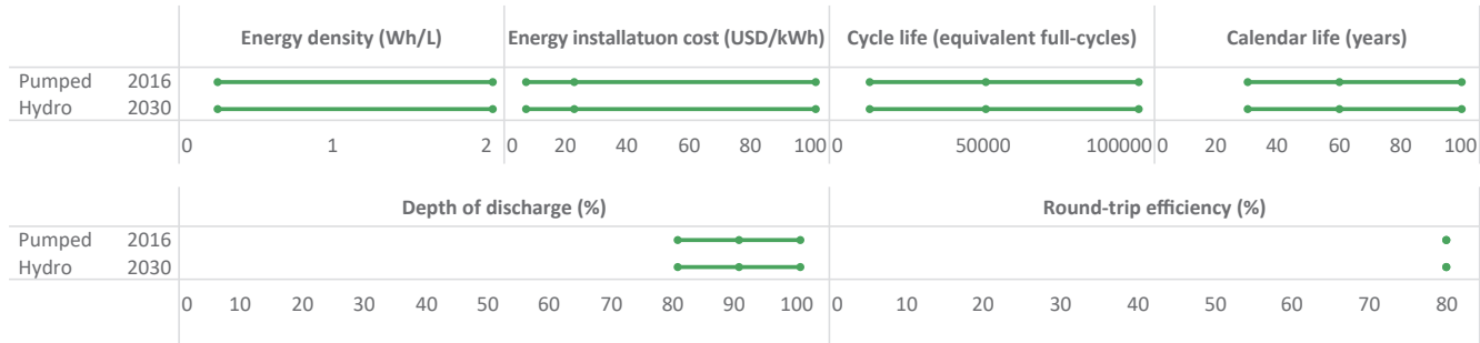
Figure 16: Properties of pumped hydro storage systems, 2016 and 2030
