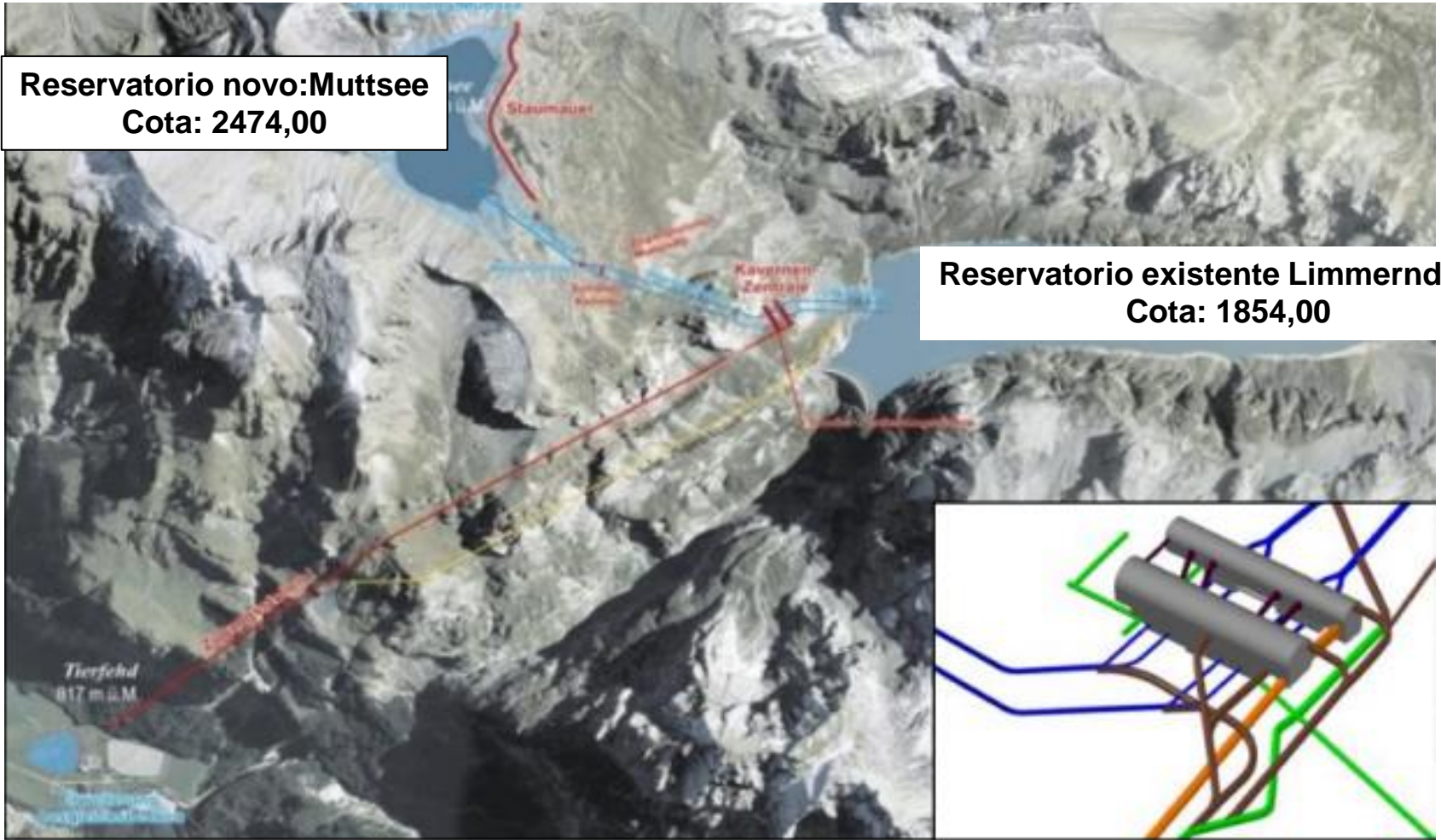
General overview of Limmern Pump Storage Power Plant, 3D-Layout of Powerhouse Cavern
