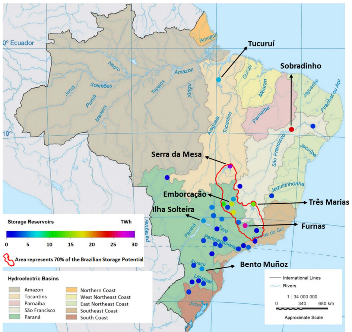
Fig. 5. Brazilian hydropower storage reservoirs highlighting an area with 70% of this potential [50].
