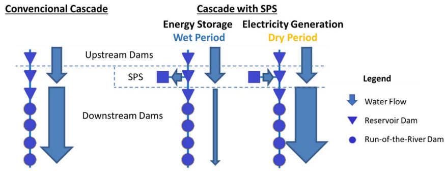
Fig. 10. Operation of (a) conventional hydroelectric plants (b) SPS during periods of high water availability (c) SPS during periods of low water availability.
