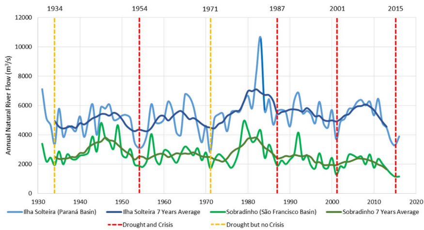
Fig. 4. Annual natural river flow time series of Ilha Solteira and Sobradinho and the energy crises in Brazil.
