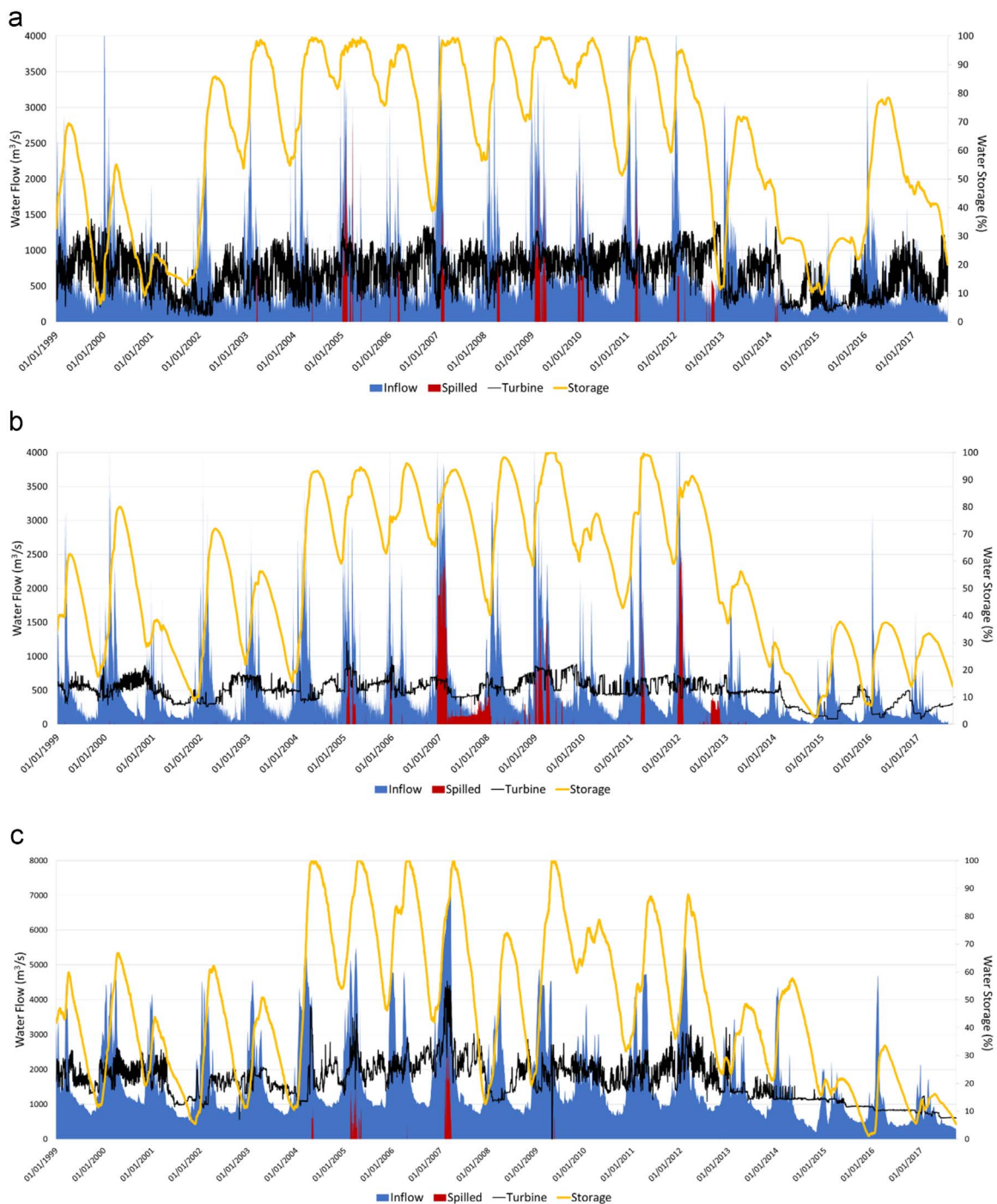
Fig. 3. Inflow, spilled and turbine flows (m 3 /s), and energy storage (%) for (a) Furnas, (b) Três Marias (c) and Sobradinho Reservoirs.
