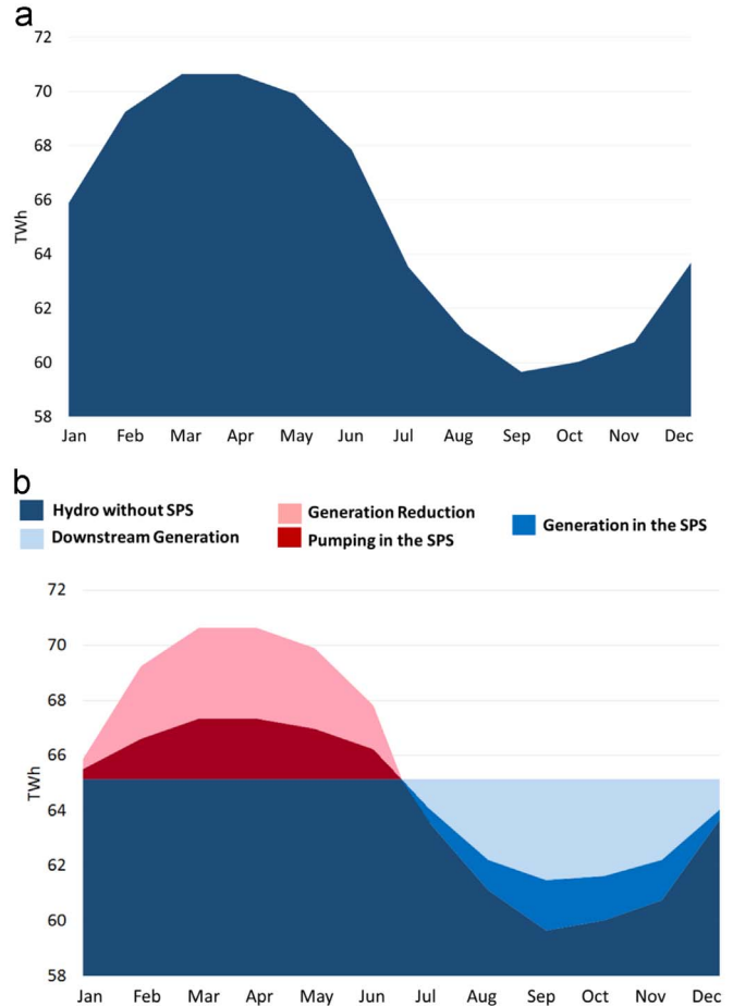
Fig. 11. Estimated hydropower generation for 2023 (a) without SPS (b) and with SPS [97].
