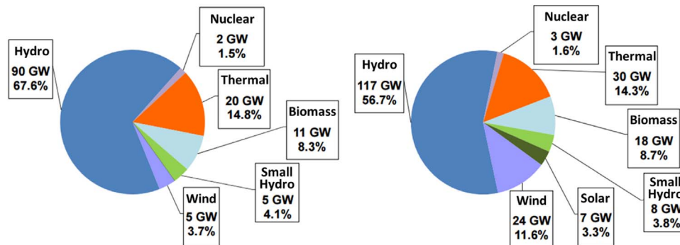
Fig. 9. Brazilian generation capacity in (a) 2014 and (b) prediction for 2024 [51].
